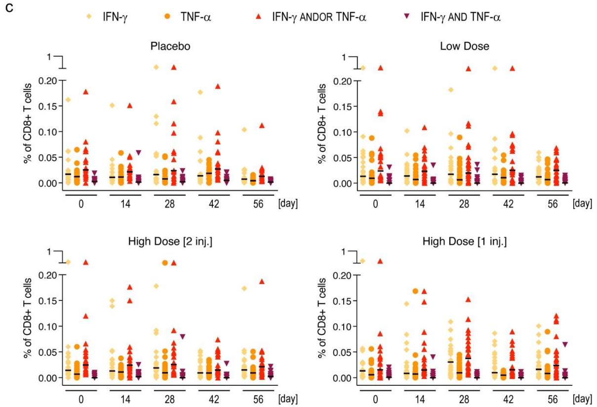
Supplementary Figure: CD4 (a and b) and CD8 (c) T cell responses to SARS-CoV-2 spike protein. T helper cells type 1 (Th1) responses (a) and T helper cells type 2 (Th2) responses (b) were characterized by analysis of cytokine production. Th1 responses were measured as CD4 T cells producing IFN- \gamma and/or TNF- \alpha , Th2 responses were measured as CD4 T cells producing IL-5 and/or IL-13. c) CD8 T cells were characterized for IFN- \gamma and/or TNF- \alpha production. PBMC from all participants (mITT set) were analyzed at the indicated time points. PBMC were stimulated with peptide pools to S1 and S2. The sum of the respective results was considered the overall response to the S protein.
