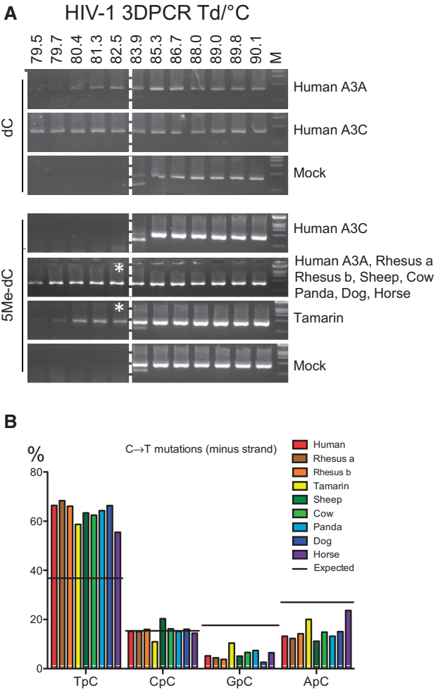
FIG. 5. A3A proteins can deaminate 5-methylcytidine in ssDNA. (A) HIV-1 specific 3DPCR gels after QT6 transfections with A3A proteins and human A3C protein along with classical dC or 5Me-dC substituted HIV-1 matrix. Asterisks denote the samples that were molecularly cloned and sequenced. (B) 5' Dinucleotide analysis of the deamination context performed on DNA minus strand for cloned PCR products.
