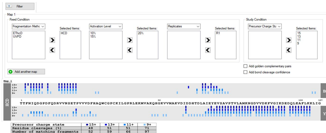
Figure 1: Screenshot of the filter interface of TDFragMapper (top panel) and the visualization module with the corresponding fragmentation map of human Thioredoxin (11 kDa) obtained when varying the precursor charge state in HCD with NCE 20% (bottom panel). Fragmentation maps obtained for larger proteins (21 and 29 kDa) are depicted in Figures S6 and S7.
