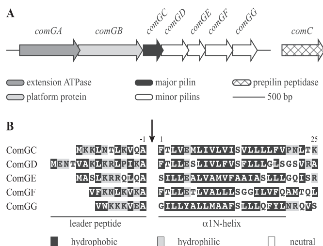
Figure 1. Com pilus machinery in S. sanguinis . A, genomic organization of the genes involved in the biogenesis of the Com pilus in S. sanguinis 2908. All the genes are drawn to scale, with the scale bar representing 500 bp. The functions of the corresponding proteins are listed at the bottom. B, sequence alignment of the putative N-terminal class III signal peptides of the five ComG pilins in S. sanguinis 2908. The 8–15-amino acid long leader peptides, which contain a majority of hydrophilic (shaded in gray) or neutral (no shading) residues, end with a conserved Ala -1 . Leader peptides are processed (indicated by the vertical arrow) by the prepilin peptidase ComC. The mature proteins start with a tract of 21 predominantly hydrophobic residues (shaded in black), which invariably form the protruding N-terminal portion of an extended \alpha -helix that is the main assembly interface within filaments.
