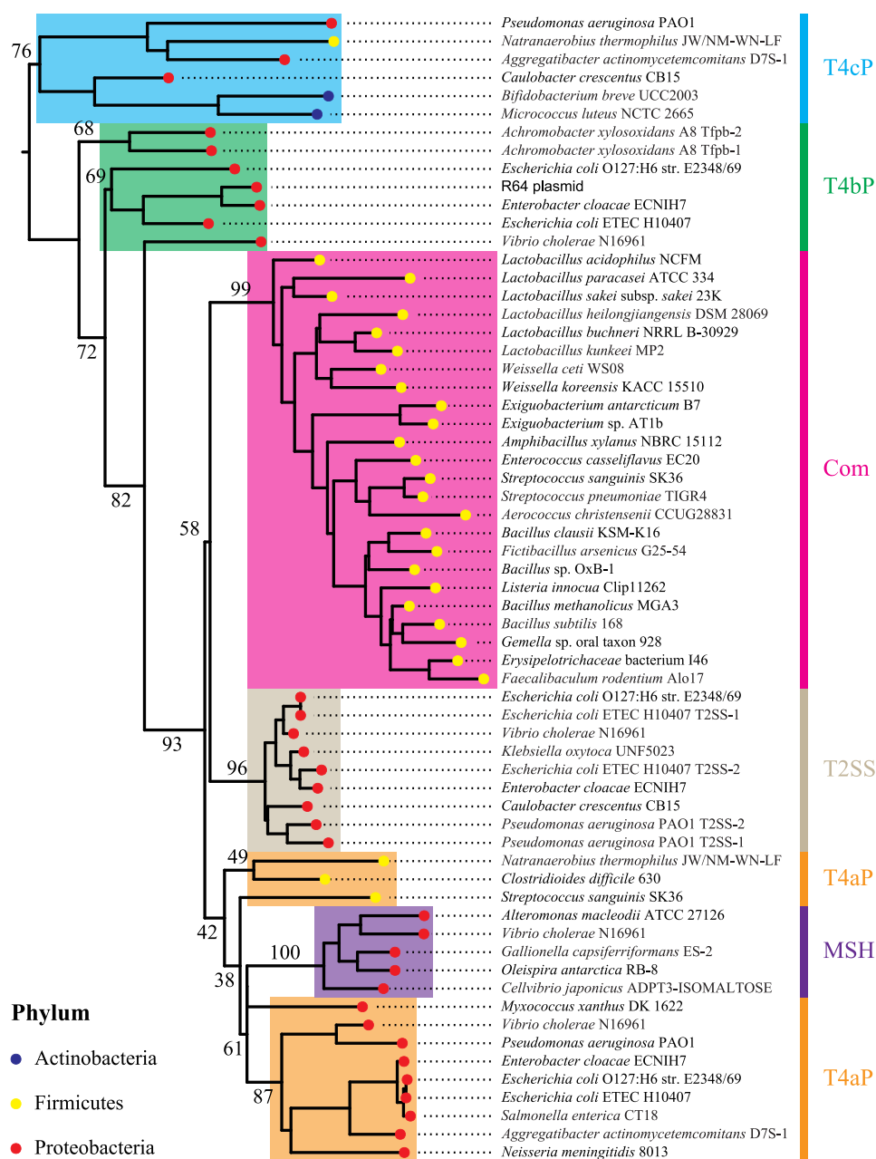
Figure 3. Rooted phylogeny of the major pilins from various bacterial T4F. The tree was build using IQ-Tree, with 1,000 replicates of UFBoot and LG + F + R4 model. Numeric values (in %) indicate UFBoot of the corresponding branches. The color of the bullet points indicates the taxonomic group of the corresponding species. The color of the strips and highlights indicate the classification of the different T4F systems. T4aP, type IVa pilus. T4bP, type IVb pilus. T4cP, type IVc pilus (also known as Tad).
