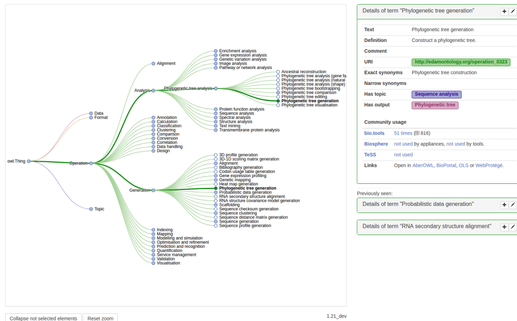
Figure 1: EDAM Browser main interface with a concept that have two parents, and relations with others concepts
