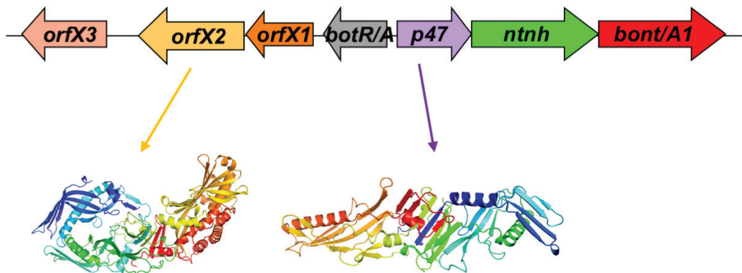
Figure 1. Genetic organization of ha-bont and OrfX-bont locus and structure of BoNT/A, NTNH, HA-NTNH-BoNT/A complex, OrfX2 and P47. L, BoNT light chain; H N , N-terminal part of BoNT heavy chain; H C , C-terminal part of BoNT heavy chain. The structure of OrfX-BoNT complex is not yet known.
