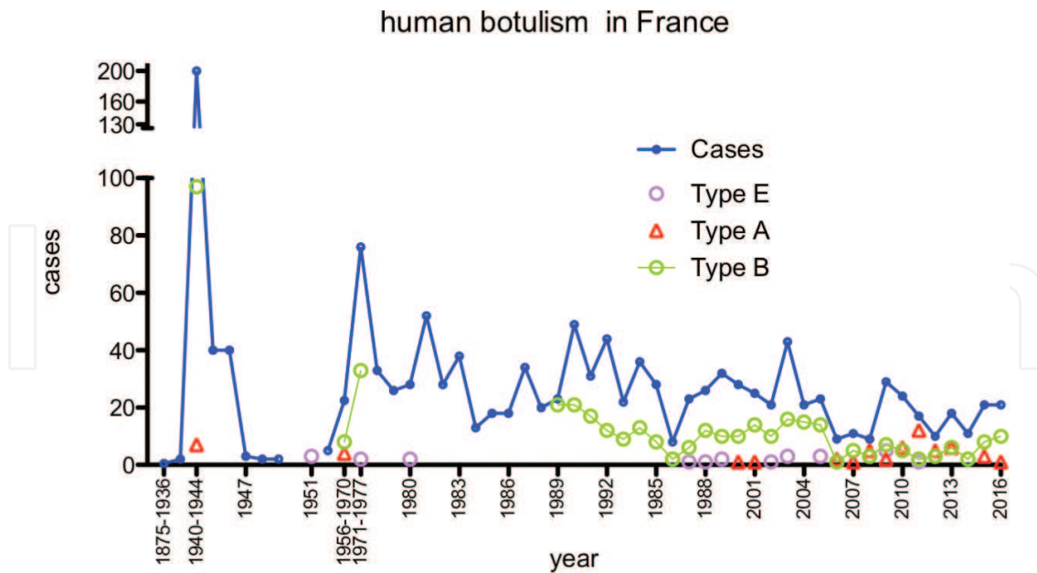
Figure 2. Incidence of human botulism in France, 1875–2016. The numbers indicated in the period ranges 1875–1936, 1940–1944, 1956–1970, and 1971–1977 are the annual mean values. Total cases (blue), type B botulism (green), type A botulism (red), type E botulism (purple), according to [127, 129–135, 147–151]. The two outbreaks of C. baratii type F botulism in 2014 and 2015 are not reported in the figure.
