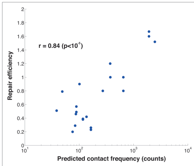
Figure 3. Computational prediction of variations in DNA repair efficiency. Experimentally measured efficiencies of homologous recombination 14 are plotted against contact frequencies predicted by our model. 17 Each of the 21 dots corresponds to a distinct pair of homologous loci (some correspond to swapped pairs). The Pearson correlation coefficient between measured efficiencies and predicted contact frequencies is 0.84.
