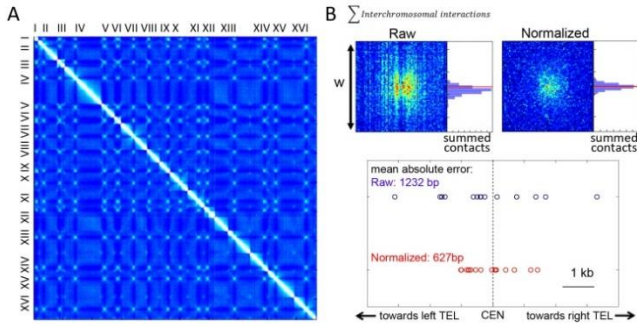
Fig. 3. (A) Normalized contact frequency matrix N_l for S. cerevisiae . (B) Summed trans -contact matrices corresponding to the submatrix of size w (Figure 2E) for chromosome 2. On the right side of each sub-matrix we plot the distribution of the centromere localizations obtained using bootstrapping. The true centromere position is indicated with a red line. The diagram below represents the distribution of the 16 centromere positions as estimated from raw and normalized data (blue and red circles, respectively). x-axis: distances along the chromosome, centered on the position of the centromere (scale bar = 1kb).
