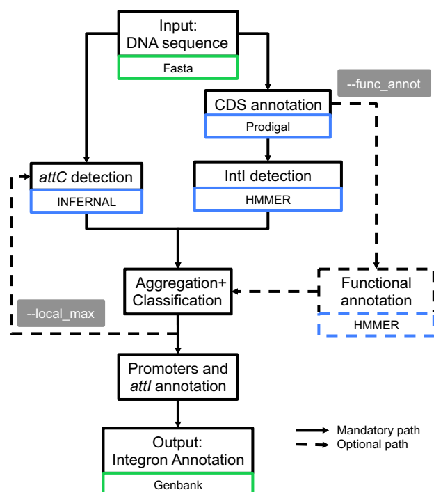
Figure 3. Diagram describing the different steps used by IntegronFinder to identify and annotate integrons. Solid lines represent the default mode, dotted lines optional modes. Blue boxes indicate the main dependency used for a given step. Green boxes indicate the format of the file needed for a given step.
