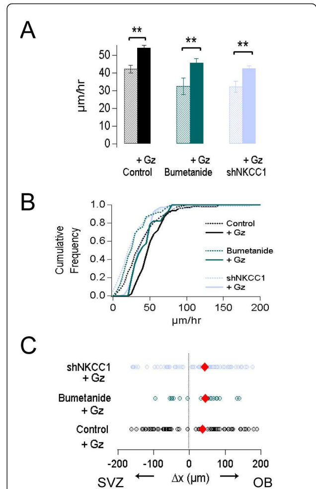
Figure 4 NKCC1 affects migration of neuroblasts in a \text{GABA}_A -independent manner. (A) Plot of the average migration speed of neuroblasts from the control, bumetanide and shNKCC1 groups (hatched bars) and these groups after incubation in 10 \mu\text{M} gabazine (+Gz; solid bars). Error bars indicate standard error of the mean. (B) Normalized cumulative plot for the averaged migration speed in the groups displayed in (A). The shift to the leftward direction in the bumetanide and shNKCC1-transduced cells treated with gabazine compared to the gabazine treated control group indicates \text{GABA}_A -receptor-independent effects (solid lines). (C) Analysis of the directionality of the migration during the experimental session in control, bumetanide-treated and shNKCC1-transduced cells incubated in gabazine. Analysis of directionality of migration as in Figure 3C.
